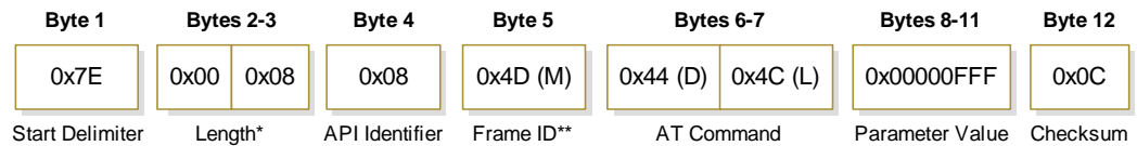
Figure 3-07. Example: API frames when modifying the DL parameter value of the modem.
