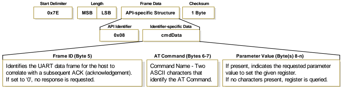
Figure 3-06. Example: API frames when reading the DL parameter value of the modem.
