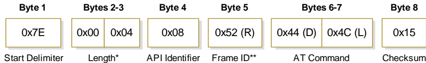
Figure 3-06. Example: API frames when reading the DL parameter value of the modem.
